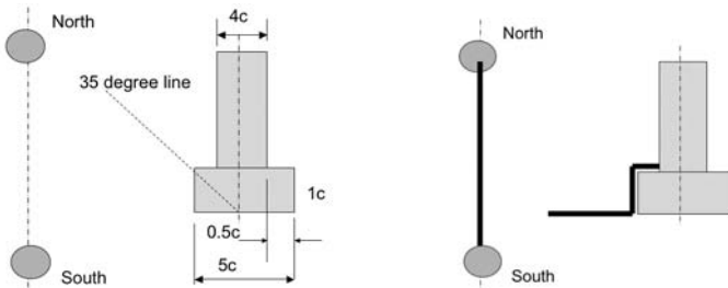
Shadows of the pillars to the bases. At the time of the winter solstice, the shadow extended the length of the distance between the two pillars (right)
